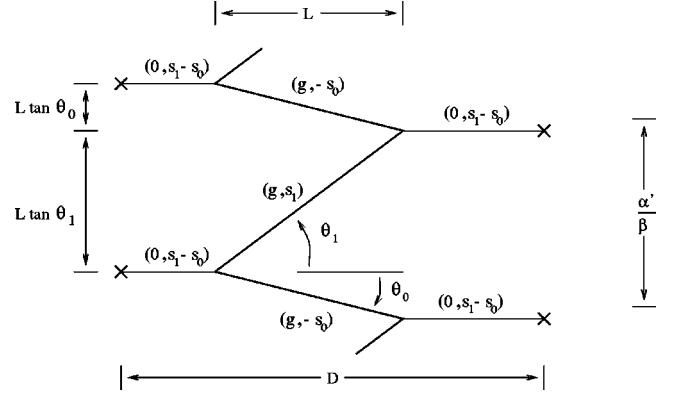
FIG. 1. String web picture of SU(2) single caloron case.
